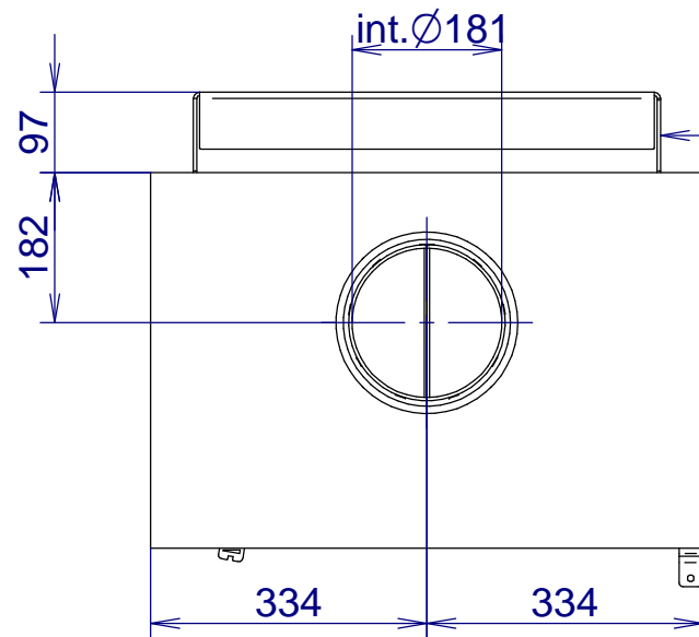
VENUS 630DC V23 in the box + console for wall
